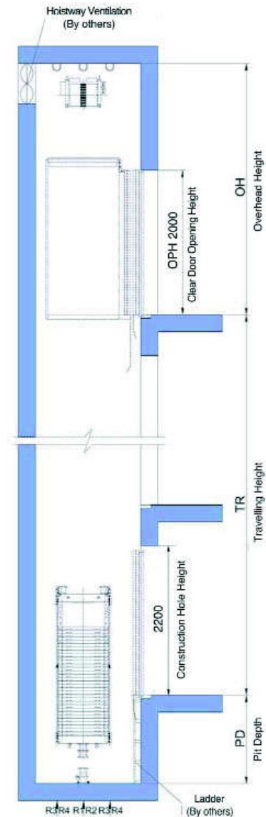
HOISTWAY TOP PLAN
